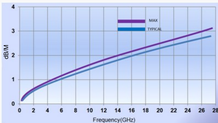
Cable Attenuation (Nominal Values @ +25 °C Ambient temperature)
