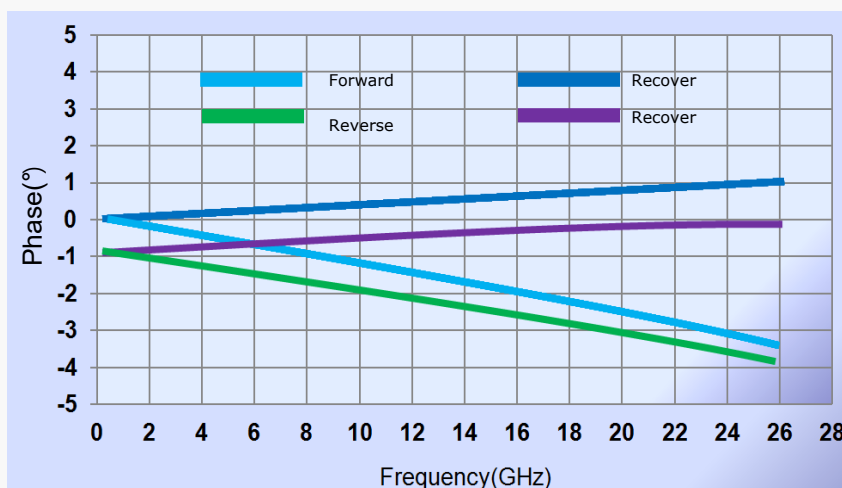
Mechanical Phase Stability
