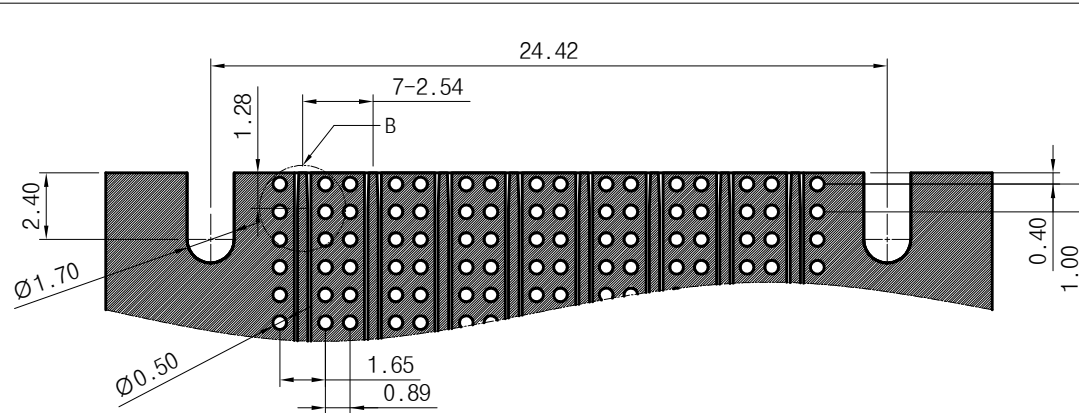
PCB Pattern
