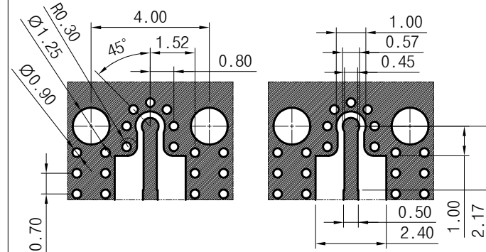
<Detail B-1> via Dimension
