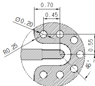
Detail A-1 Via Dimension
