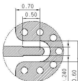
Detail A-2 Top pattern Dimension
